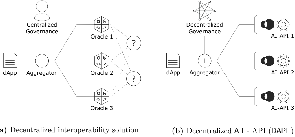
Figure 2: Decentralized interoperability solutions employ third-party oracles that do not natively reveal their sources. DAPIs are composed of first-party oracles, meaning that AI-API providers operate their own Airnodes. In addition, DAPIs are decentralized in how they are governed, resulting in end-to-end decentralization.
